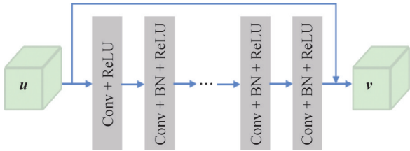
图4 去噪模块网络架构 Fig. 4 Network architecture of the denoising module
